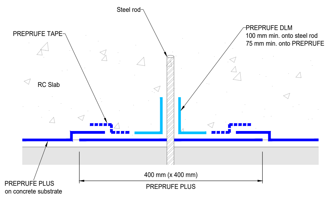
A STEEL ROD PENETRATION THROUGH SLAB Section
