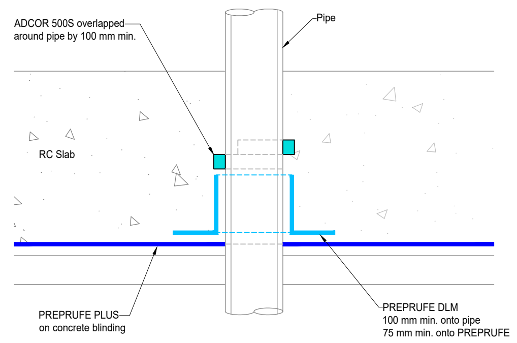
B PIPE PENETRATION THROUGH SLAB Section
