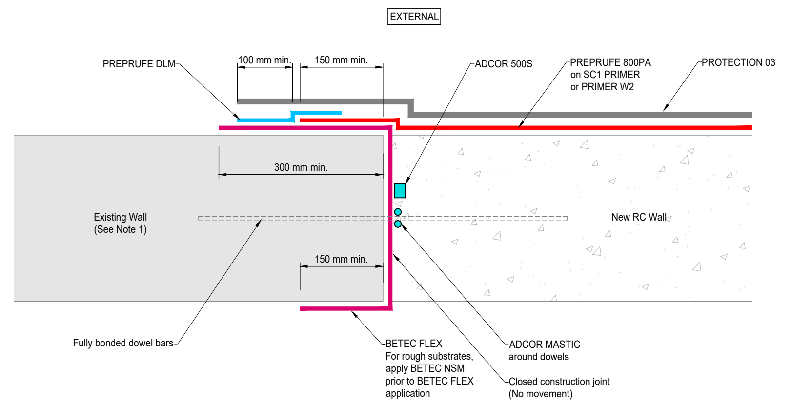
A NEW TO EXISTING WALL CONSTRUCTION JOINT Plan Section
