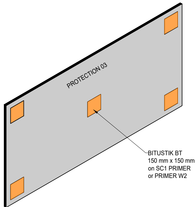
B PROTECTION 03 - BITUSTIK BT PATCH APPLICATION Isometric
