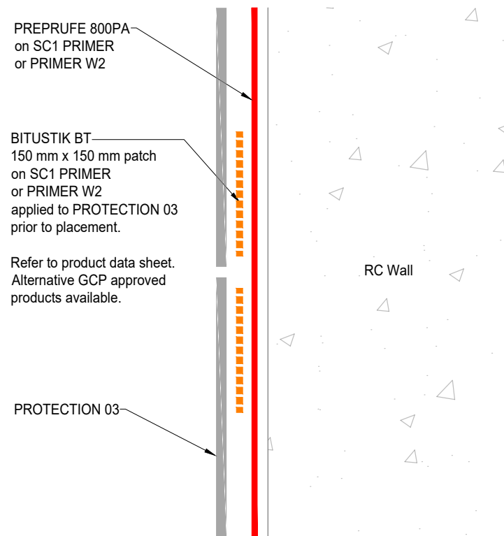
A PROTECTION 03 LOCATED WITH BITUSTIK BT PATCHES Section
