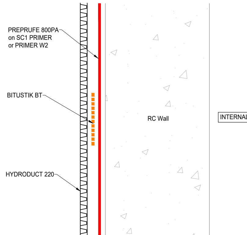
C HYDRODUCT 220 LOCATED WITH BITUSTIK BT Section
