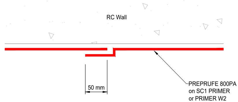
B-B VERTICAL OVERLAP Plan Section
