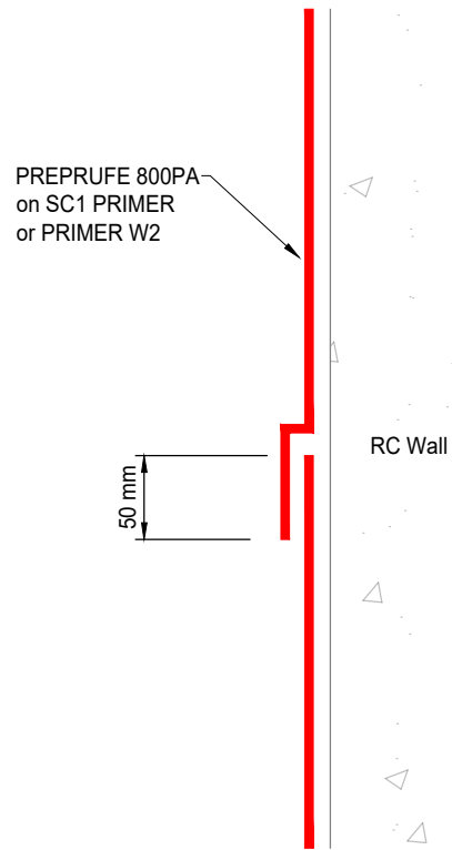
A-A OVERLAP Section
