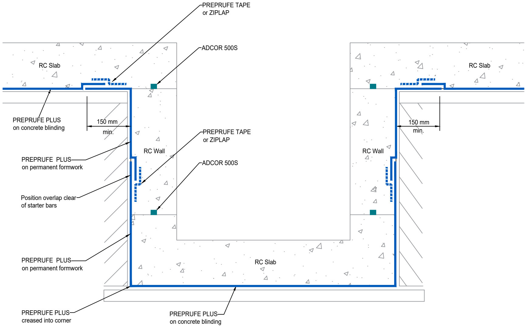
LIFT PIT Section
