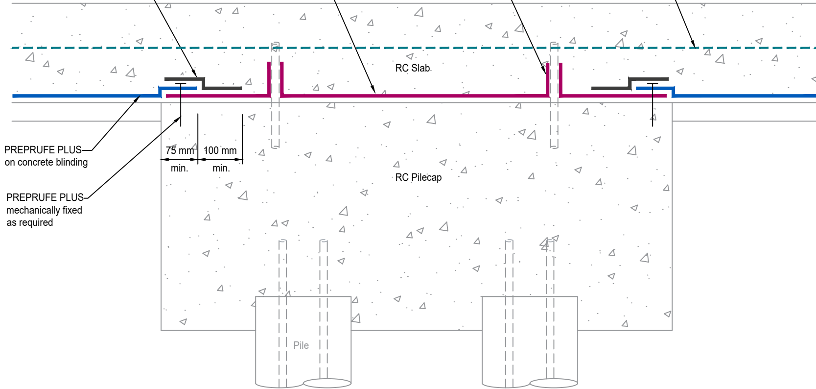
ALTERNATIVE APPLICATION OVER PILECAP Section
