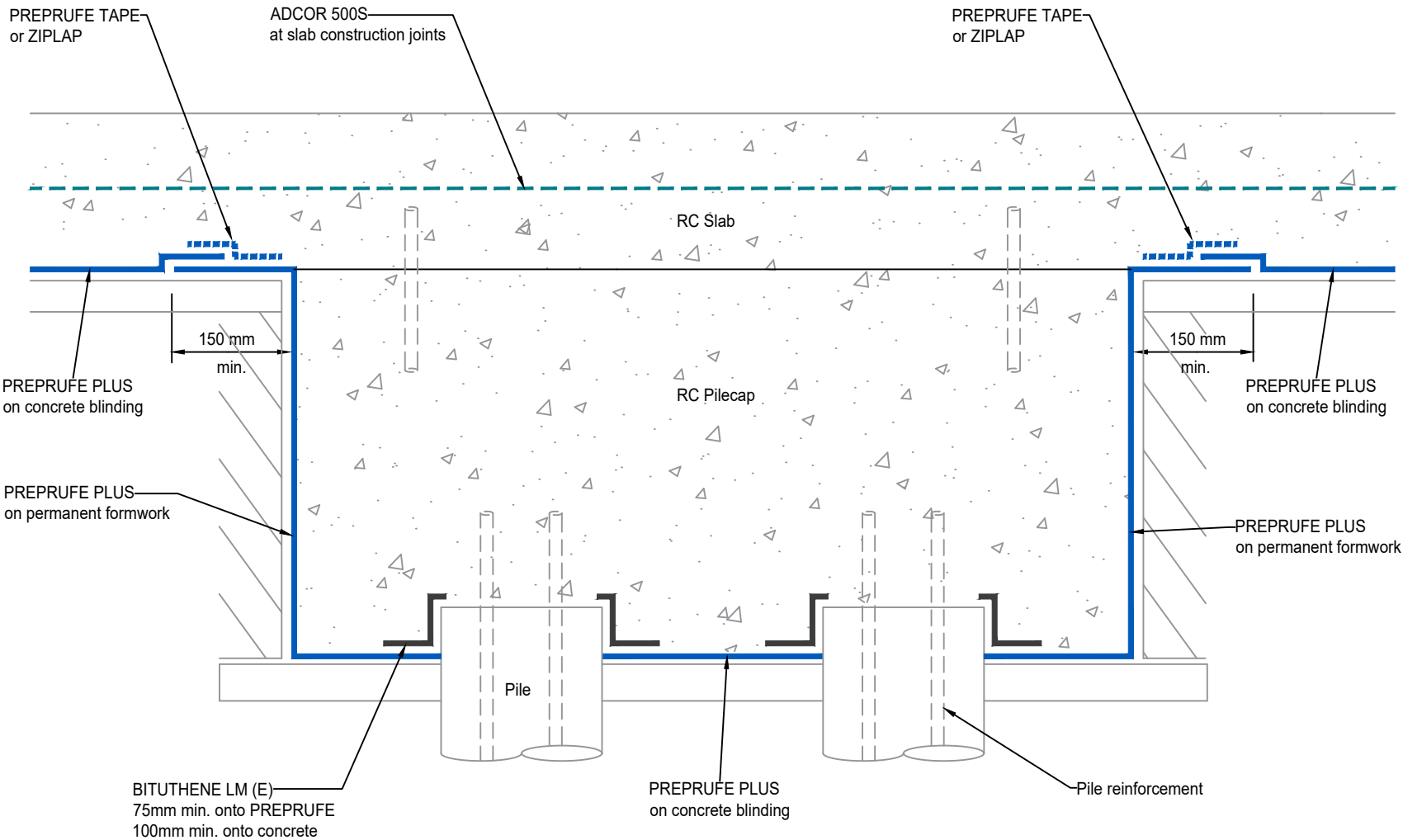
PILECAP Section
