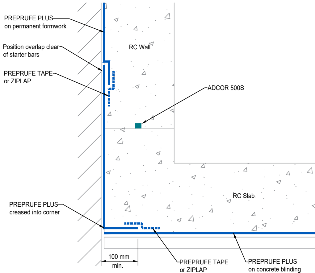
SLAB / WALL INTERFACE AGAINST PERMANENT FORMWORK Section
