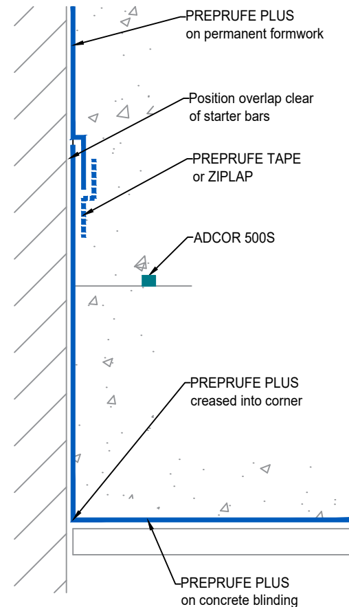
ALTERNATIVE PREPRUFE CONFIGURATION Section
