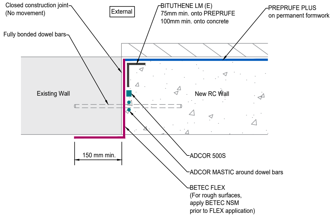
NEW TO EXISTING WALL CONSTRUCTION JOINT Section
