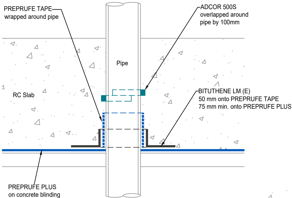
PIPE PENETRATION THROUGH SLAB Section
