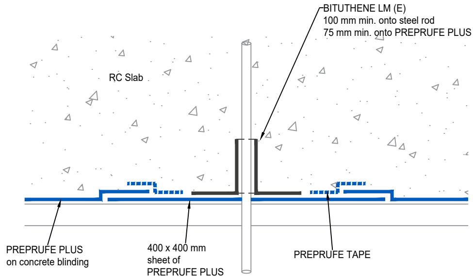
STEEL ROD PENETRATION THROUGH SLAB Section
