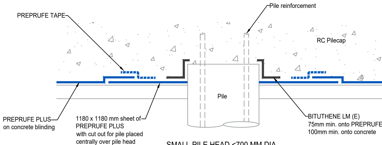
SMALL PILE HEAD <700 MM DIA. Section
