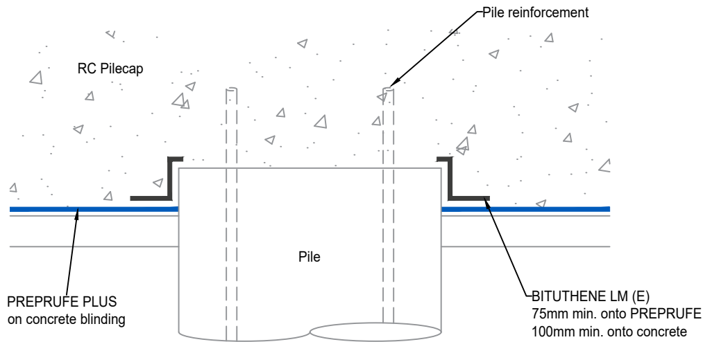
PILE HEAD Section
