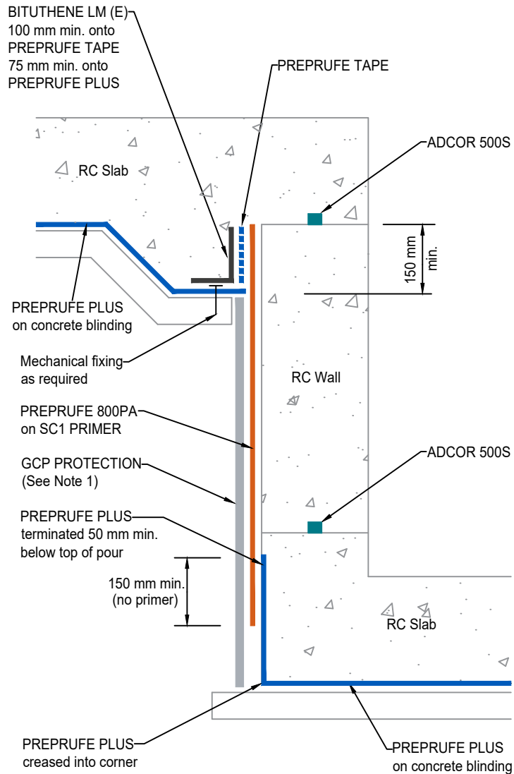
OPTION A Section
