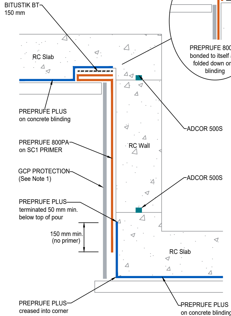
OPTION B Section
