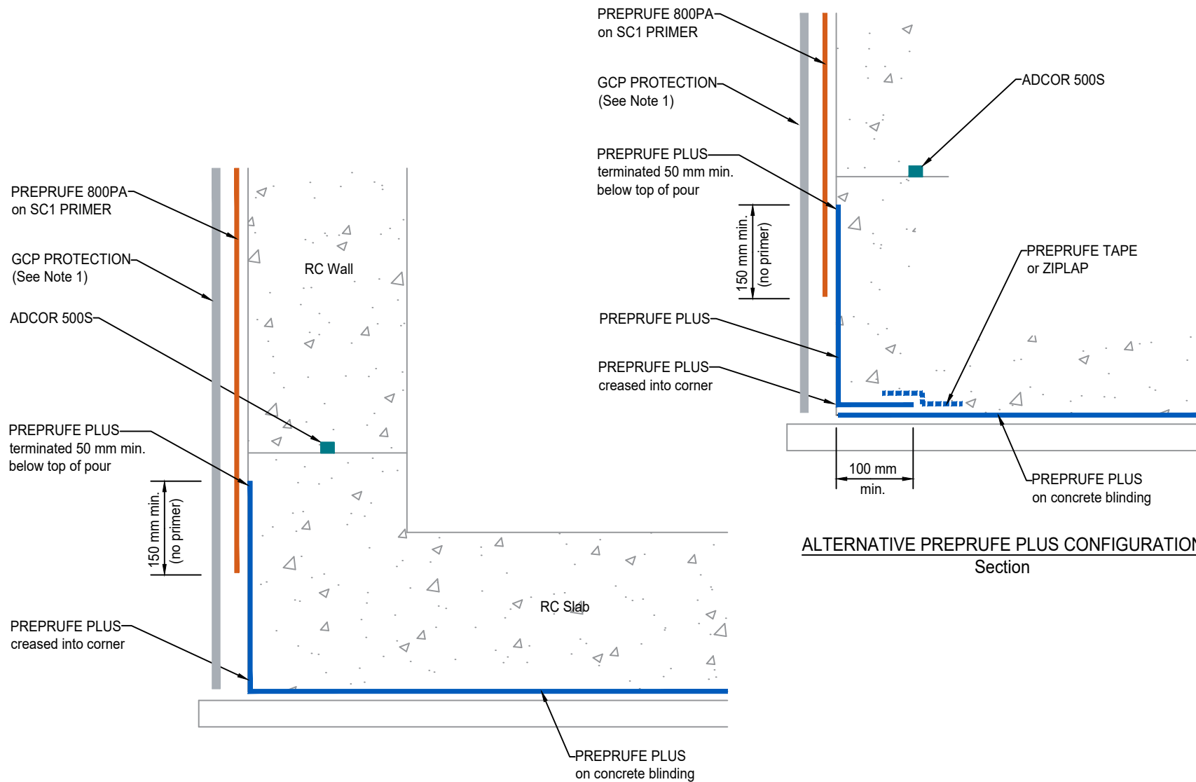
SLAB / WALL INTERFACE - REMOVABLE FORMWORK Section
