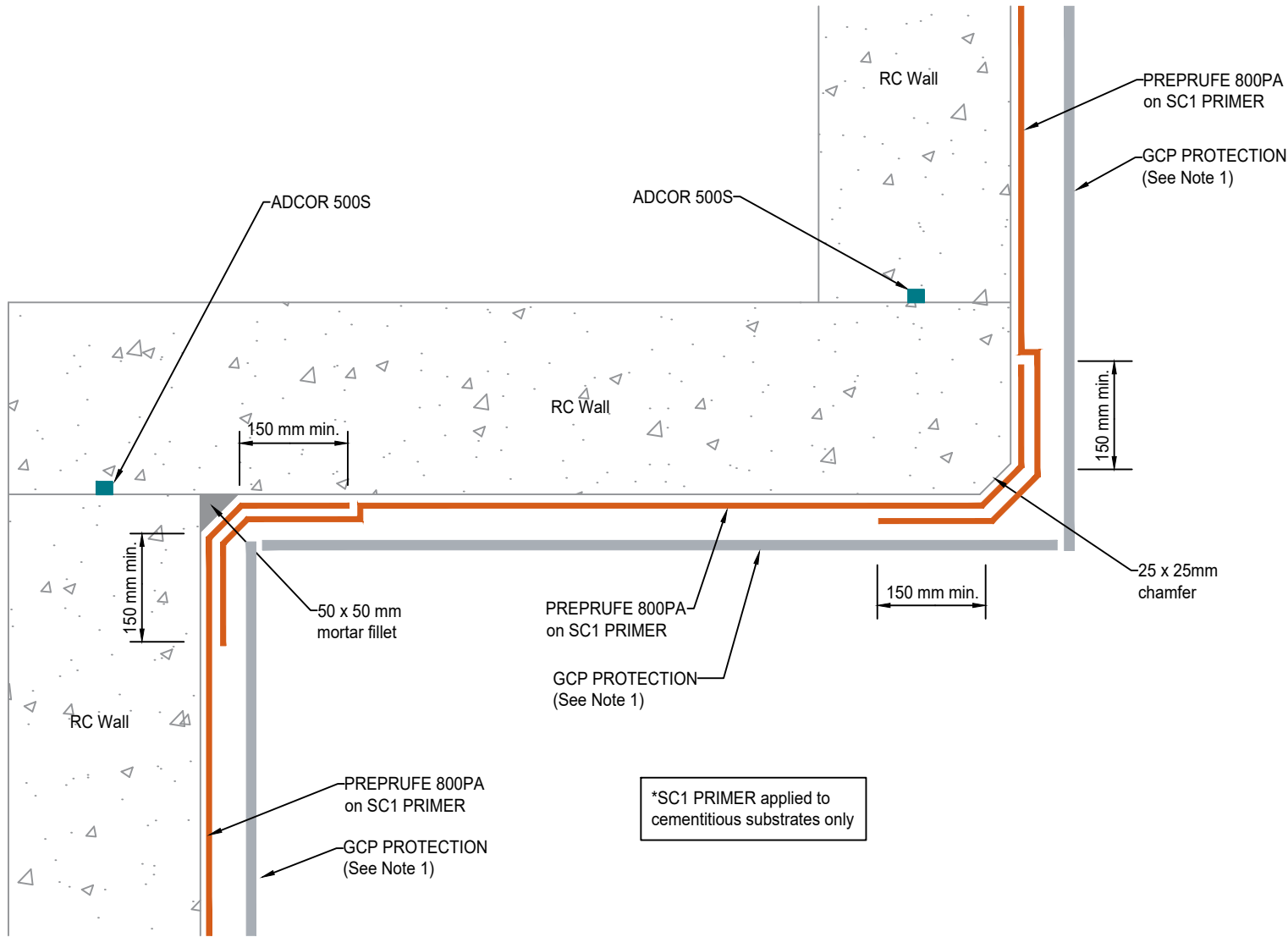
VERTICAL INTERNAL & EXTERNAL CORNERS Plan Section
